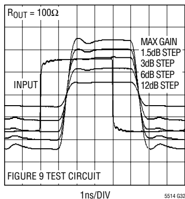
Pulse Response vs Attenuation, LT5514 Levels are: V_{IN} = 66\text{mV}_{P-P} , V_{OUT} = 2V_{P-P} at Max Gain
