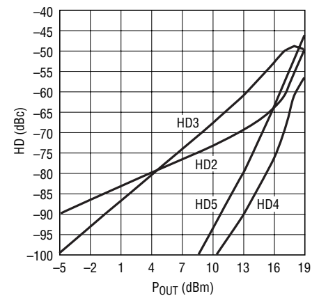
Harmonic Distortion vs P_{OUT} at 50MHz, Max Gain, R_{OUT} = 100\Omega
