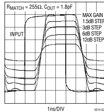
Pulse Response vs Attenuation, LT5514 Levels are: V_{IN} = 66\text{mV}_{P-P} , V_{OUT} = 4V_{P-P} at Max Gain
