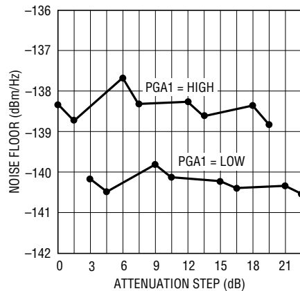
Output Noise Floor vs Attenuation Step, Freq = 100MHz, R_{OUT} = 200\Omega
